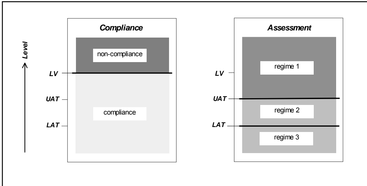
Figure 9.1. Implication of exceedance of the limit value (LV), the upper assessment threshold (UAT) and the lower assessment threshold (LAT) for compliance judgement and requirements in a zone
